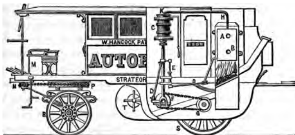
FIG. 49.—Hancock's "Autopsy," 1838.
